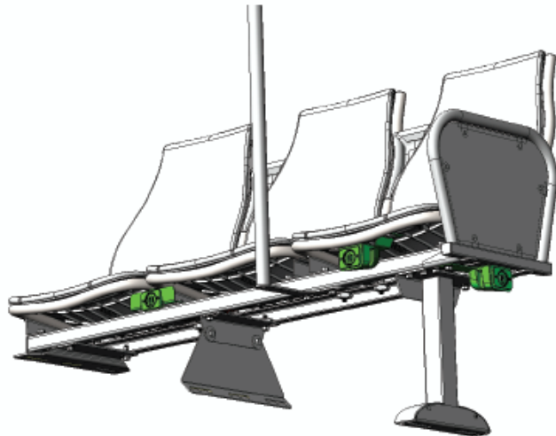
3P Longitudinal w/ Stanchion
