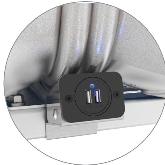
Rear Mount
