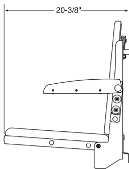
Cantilever Mount
