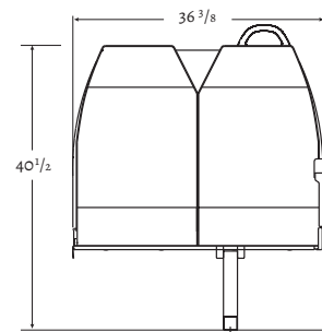
T-Pedestal Mounting
