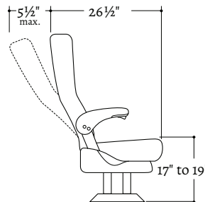
Recline Range Adjustable (0°-5½°)
